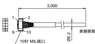
ON/OFF输入用线缆 EXCB2-M10-3(3m)
